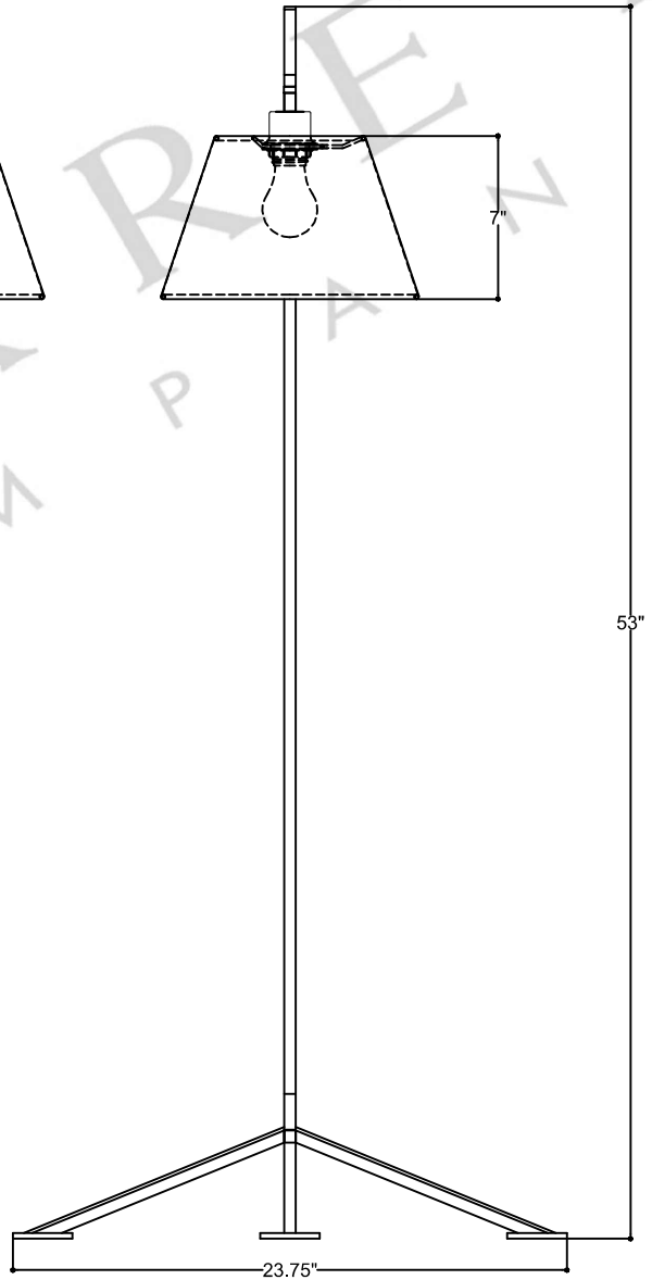
FRONT VIEW
